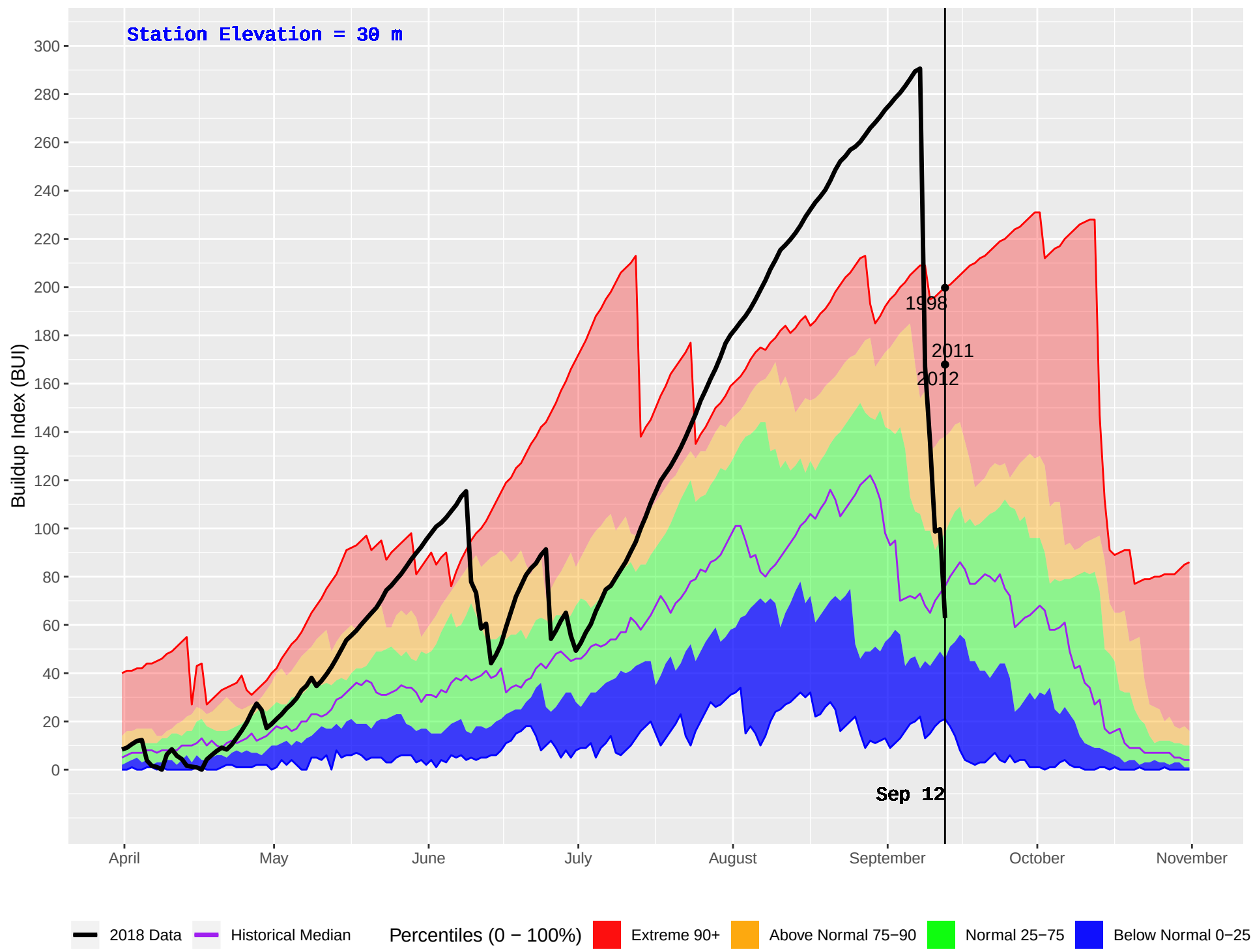
CEDAR (59) : Historical (1989–2016) and Current (2018) Daily Buildup Index (BUI)
