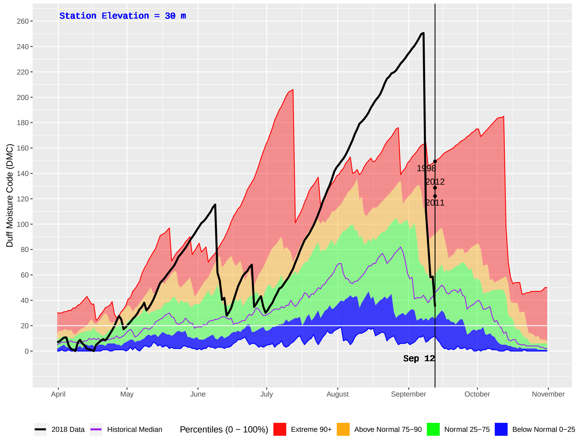
CEDAR (59) : Historical (1989–2016) and Current (2018) Daily Duff Moisture Code (DMC)
