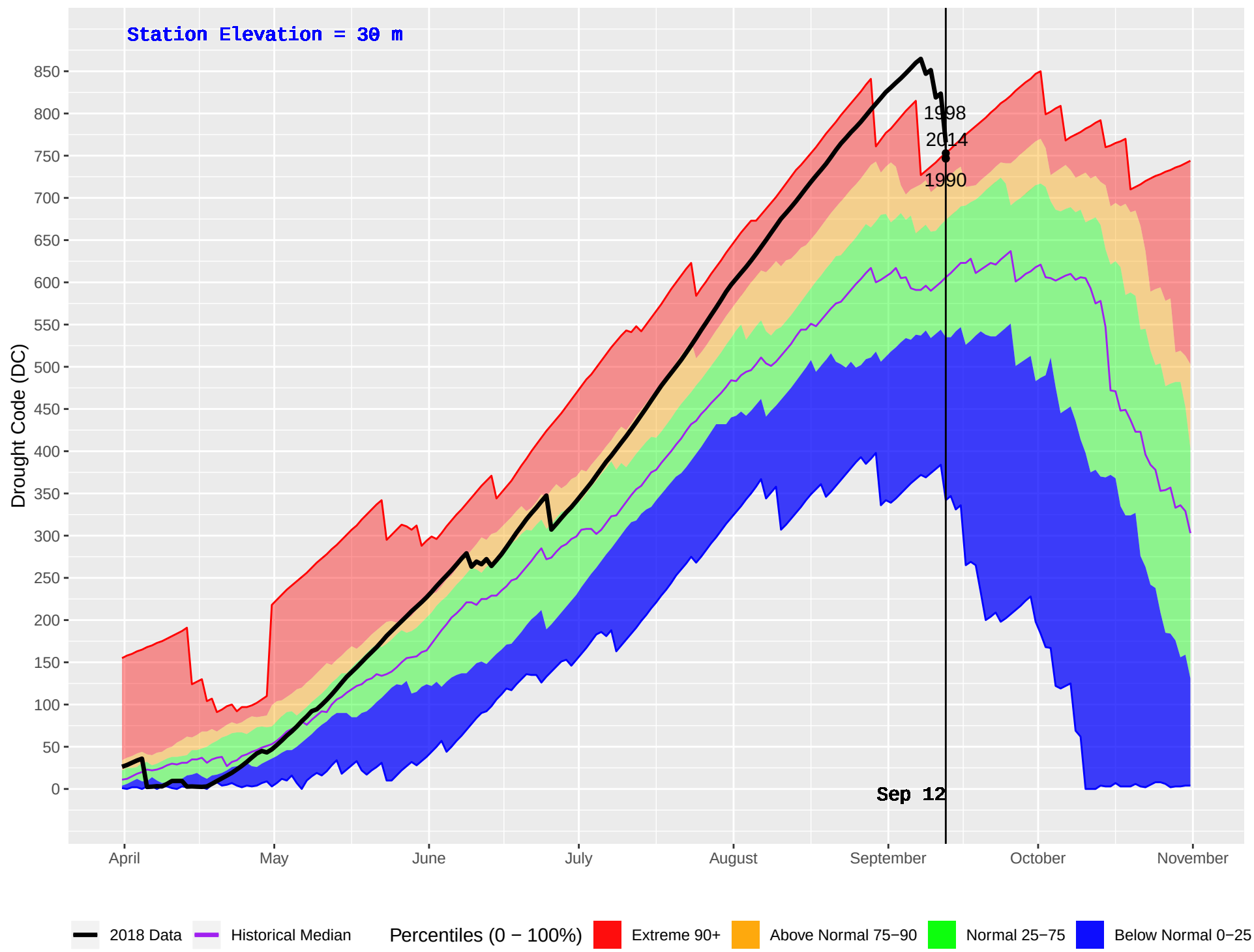
CEDAR (59) : Historical (1989–2016) and Current (2018) Daily Drought Code (DC)
