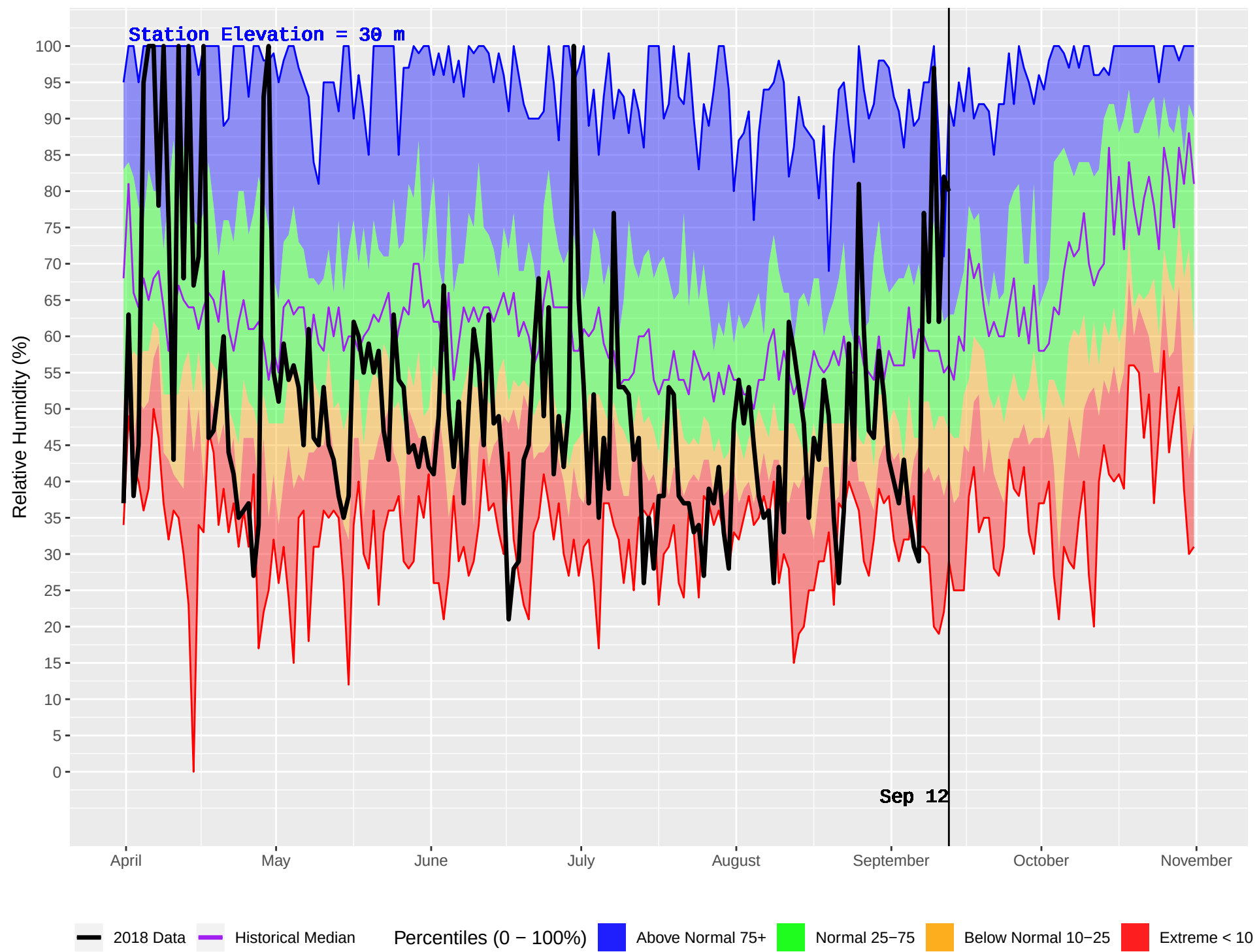
CEDAR (59) : Historical (1989–2016) and Current (2018) Daily Relative Humidity
