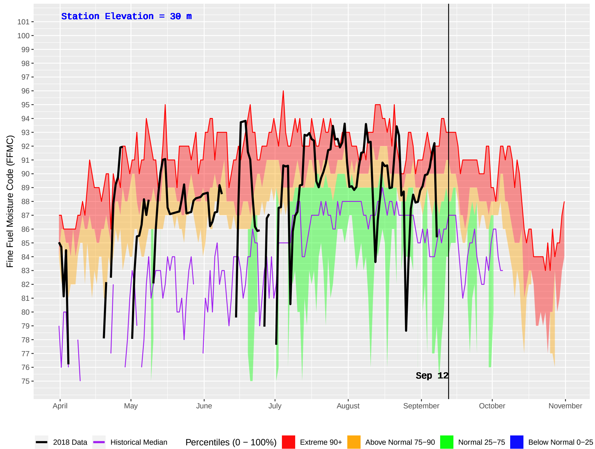
CEDAR (59) : Historical (1989–2016) and Current (2018) Daily Fine Fuel Moisture Code (FFMC)
