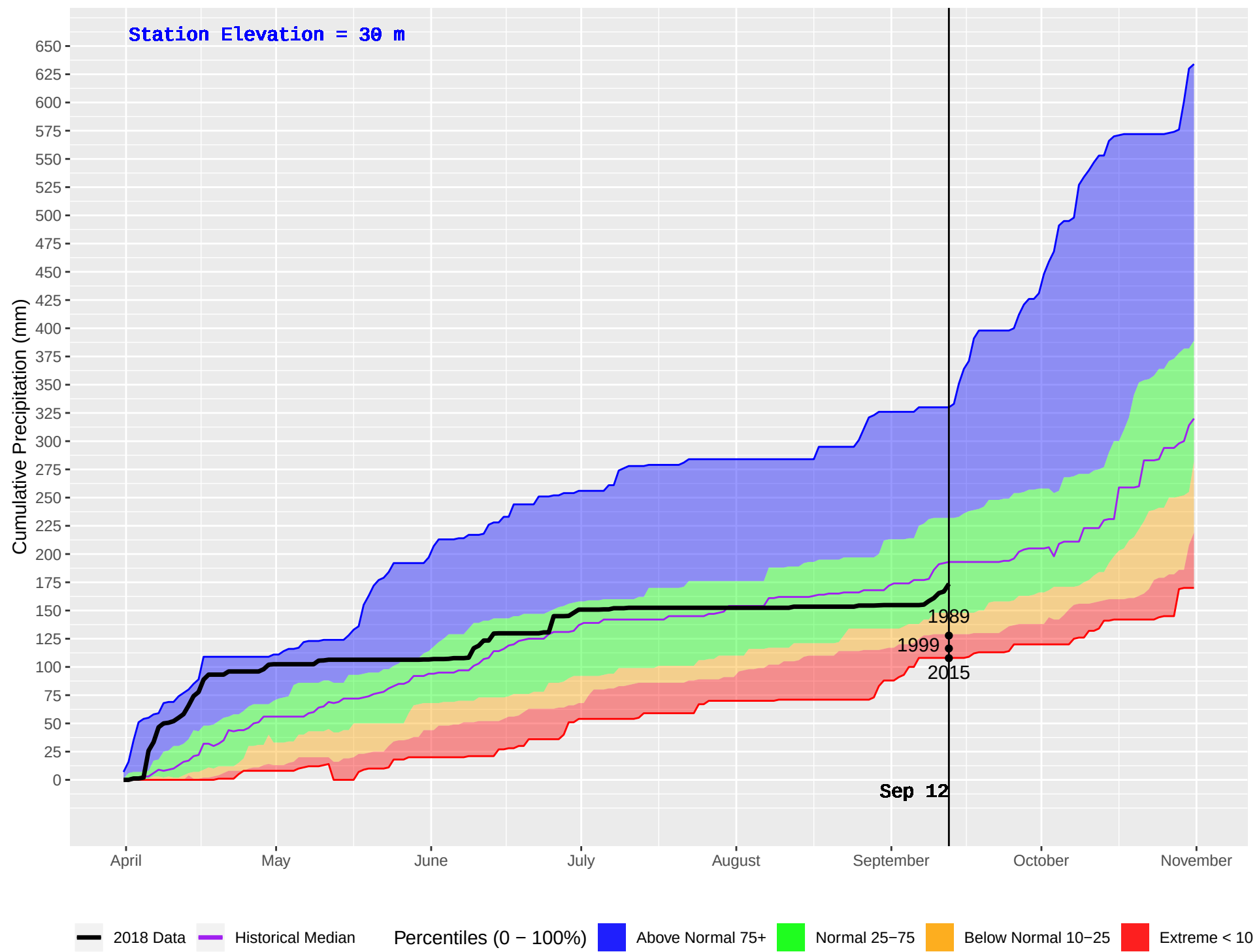
CEDAR (59) : Historical (1989–2016) and Current (2018) Daily Cumulative Precipitation
